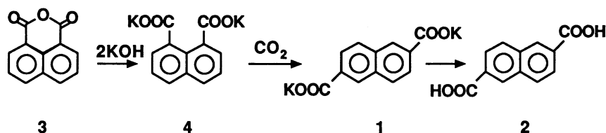
Scheme 1. Henkel process.
